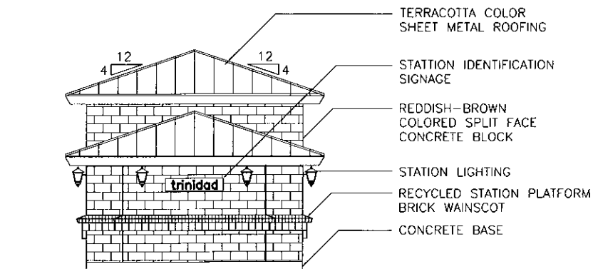
WEST SIDE ELEVATION SCALE 3/16"=1'-0"
