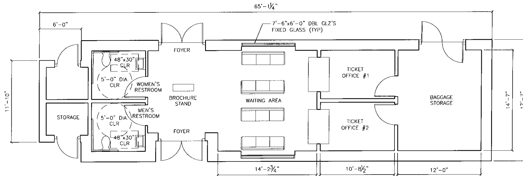
PROPOSED FLOOR PLAN SCALE 1/4"=1'-0"
