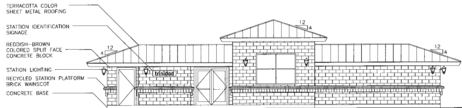
SOUTH SIDE ELEVATION SCALE 3/16"=1'-0"
